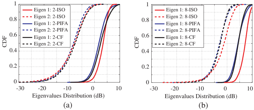
Figure 11. Eigenvalue distributions of the studied (a) 2 \times 2 and (b) 2 \times 8 MIMO systems in Route A.
