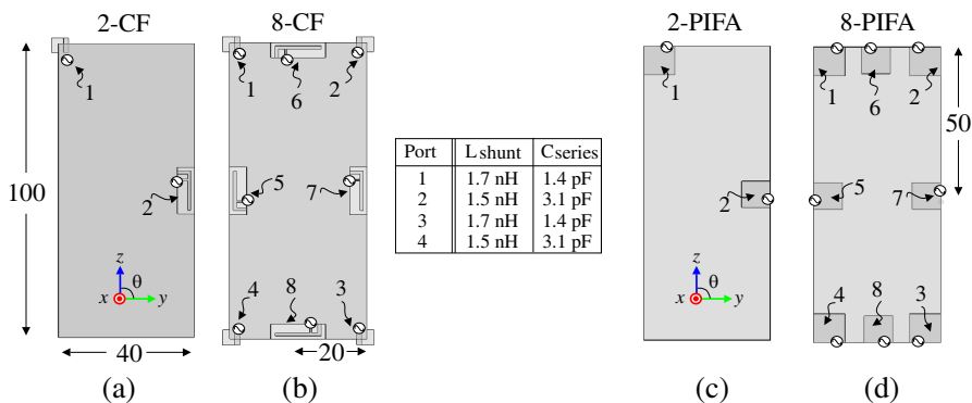
Figure 3. Proposed MA configurations (a) ‘2-CF’, (b) ‘8-CF’, and PIFA-based MA configurations as reference structure (c) ‘2-PIFA’, (d) ‘8-PIFA’. All dimensions are in millimeter.
