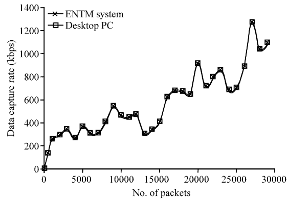
Fig. 15: Data capture rate comparison between ENTM system and desktop PC
