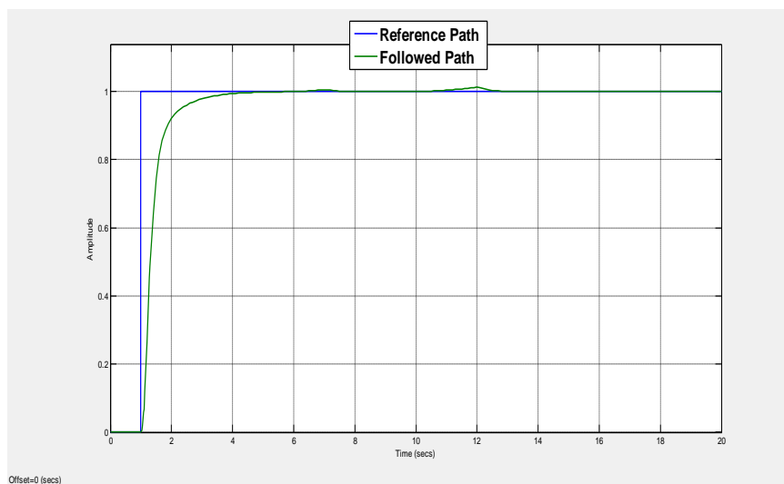
Fig. 3: Reference path and MPC effectiveness
