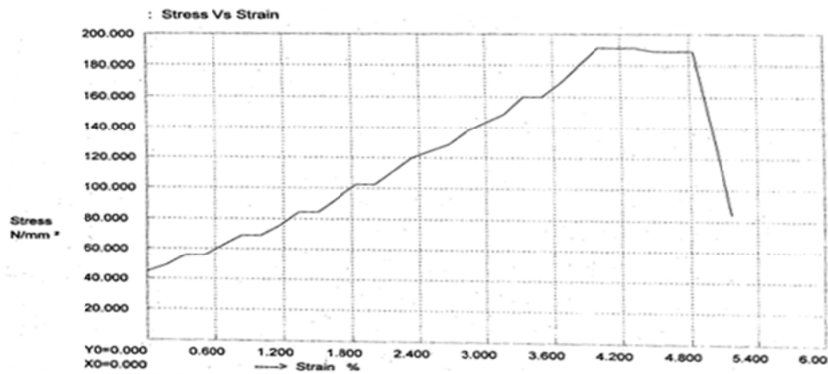
Fig. 5: Stress-Strain Curve for as-Received Composite.
