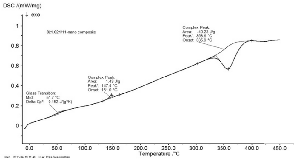
Fig. 7: DSC Graph for 5wt% Nano Composite.
