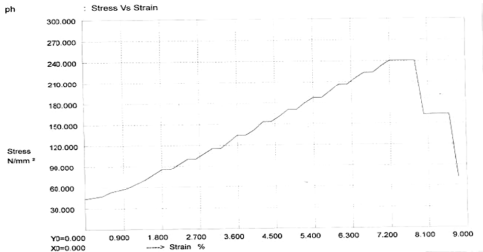
Fig. 4: Stress-Strain Curve for 5wt% Nano Composite.
