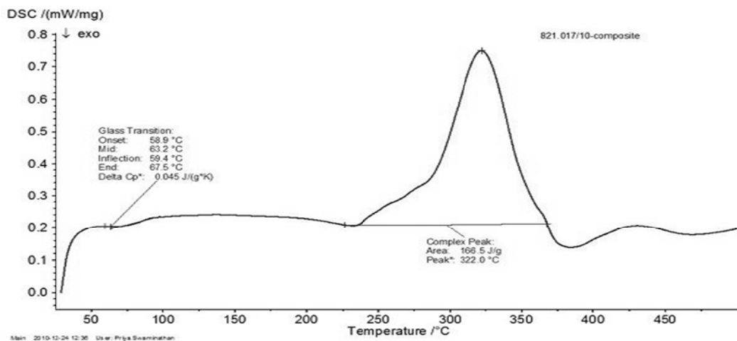
Fig. 6: DSC Graph for As-received Composite.
