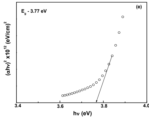
Fig. 3: (\alpha h\nu)^2 vs h\nu plots for \text{In}_2\text{O}_3 films deposited at different substrate temperatures (a) 350 (b) 400 (c) 450 (d) 500 and (e) 550 °C
