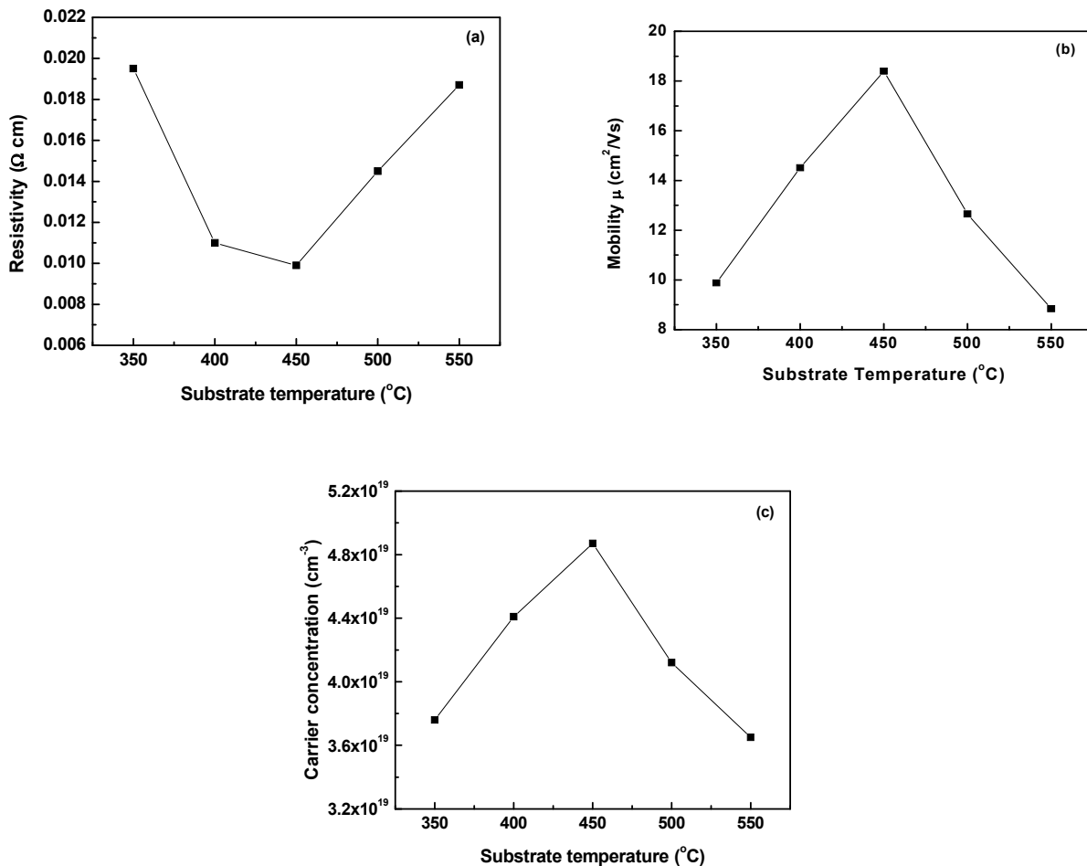
Fig 4: Variation of resistivity (a), mobility (b) and (c) carrier concentration of In 2 O 3 film with substrate temperature
