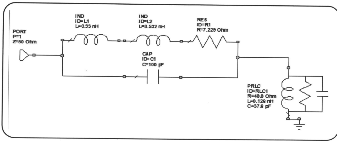
Figure 2. The equivalent circuit for coaxial probe fed microstrip patch antenna.
