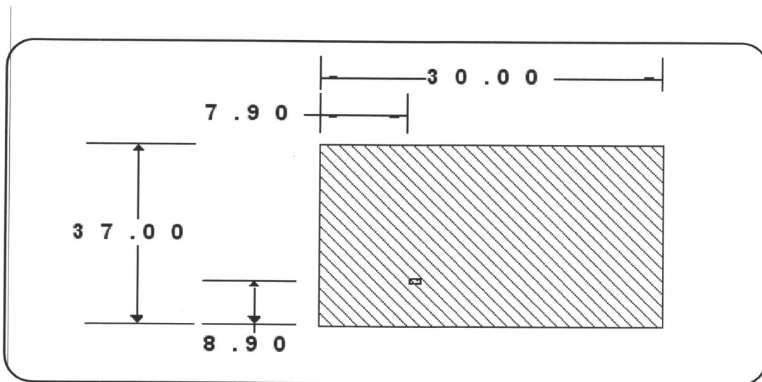
Figure 3. Dimension of the coaxial probe fed antenna.
