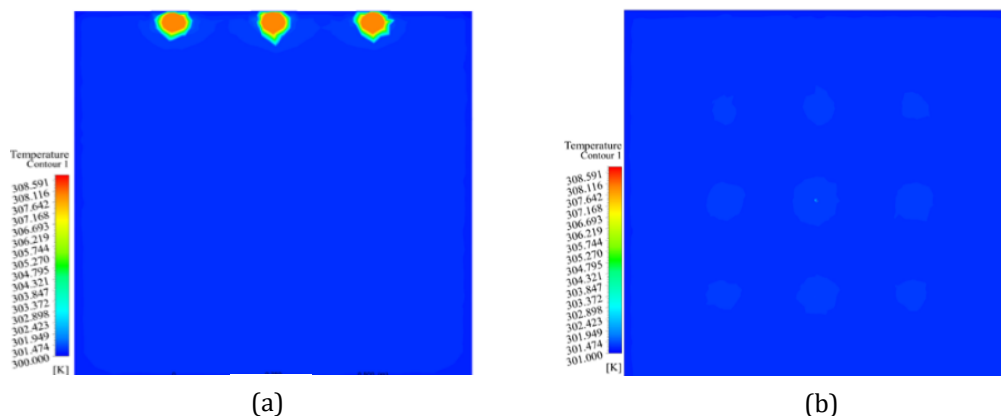
Figure 13. (a) Temperature distribution at: (a) a vertical section for 9 LED lamps; (b) a horizontal section of 10 cm away from 9 LED lamps;
