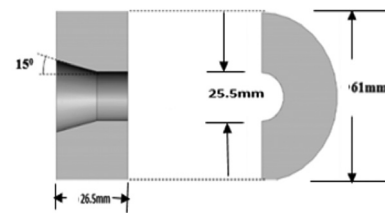
Figure 2: Front view and End view of the die at 15° entry angle
