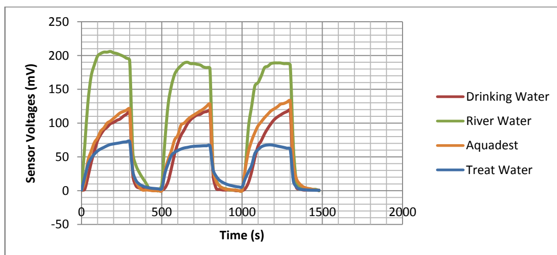
Fig. 4: The response of chitosan film sensor to different water samples.
