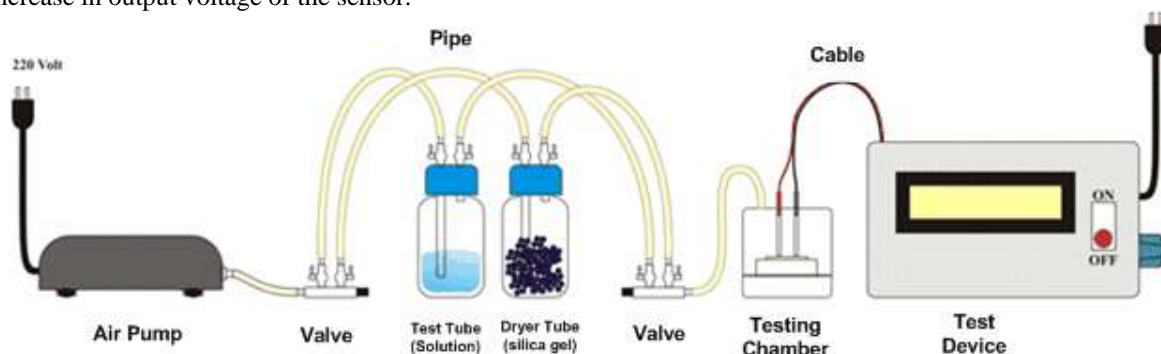
Fig. 2: Electrical testing of sensor properties scheme.
