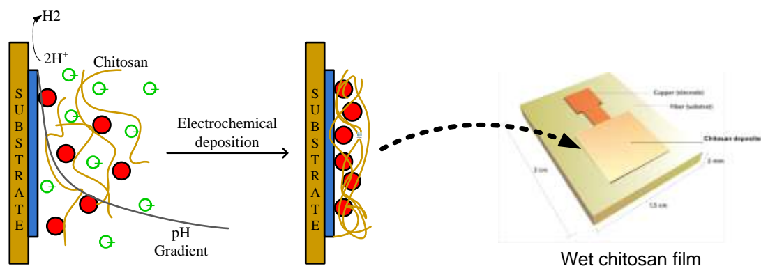
Fig. 1: Chitosan coating process with electrochemical deposition method
