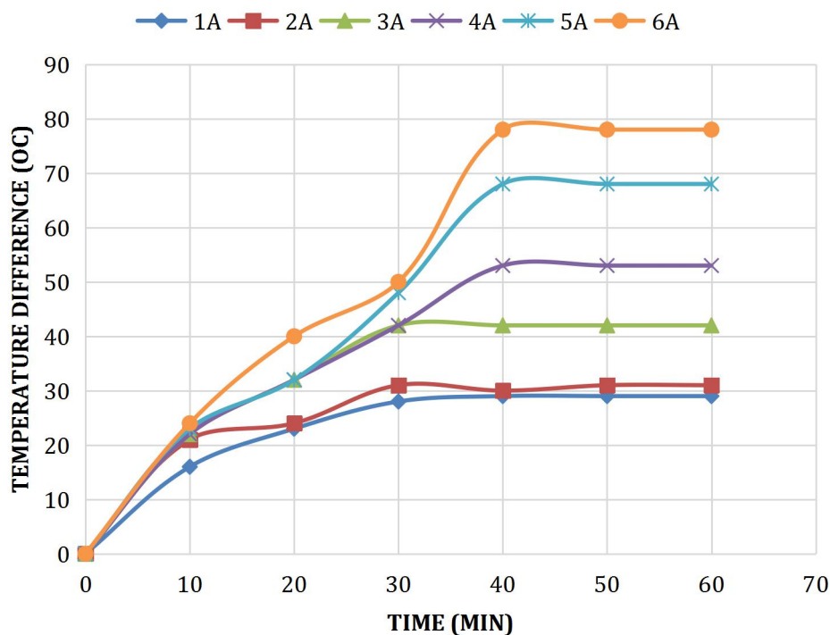
Figure 7. Graph of temperature difference between hot and cold side of TEC versus time at various current supply.
