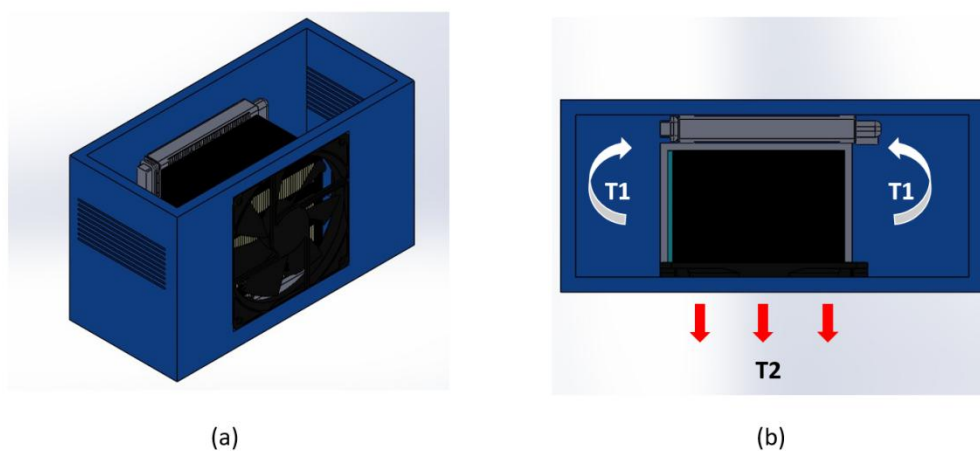
Figure 6. Isometric view of condensing system of TEC air conditioner (b) Top view of condensing system of TEC air conditioner.
