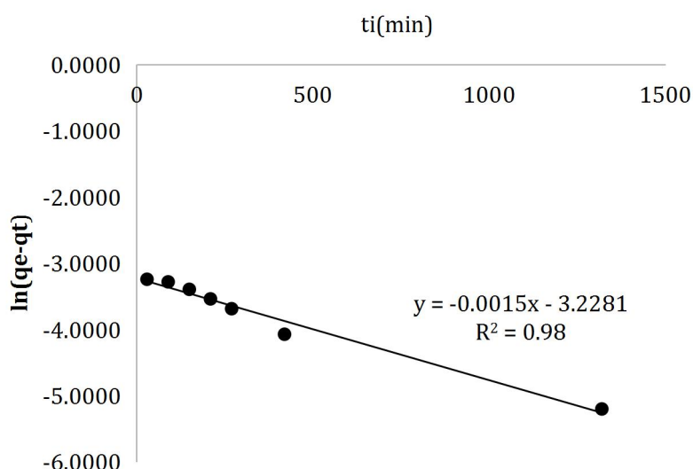
Figure 4. Pseudo First Order for \ln(q_e - q_t) versus t_i(\text{min}) .
