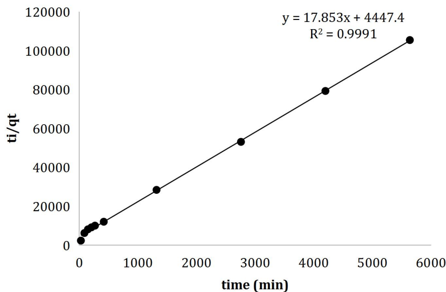
Figure 5. Pseudo Second Order for t_i/q_t versus t_i (min).
