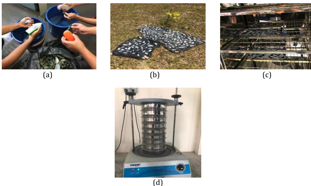
Figure 2. Preparation of the mussel shells adsorbent, (a) Cleaning of the raw materials, (b) Drying under sunlight, (c) Drying in oven (103°C to 105°C) and (d) Sieving.
